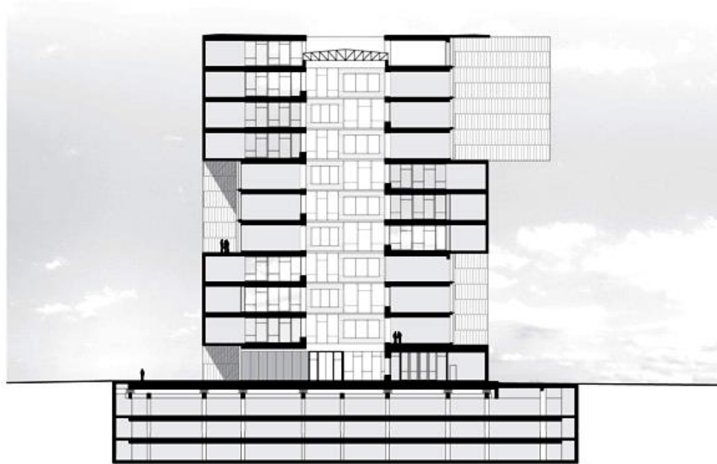
SECTION 1 - 1/500
