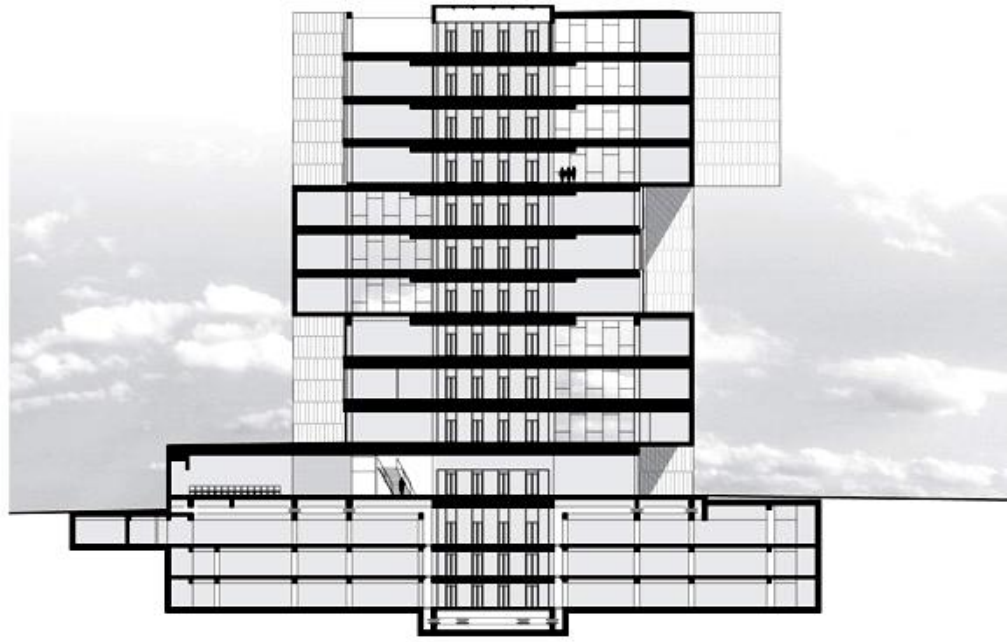
SECTION 1 - 1/500
